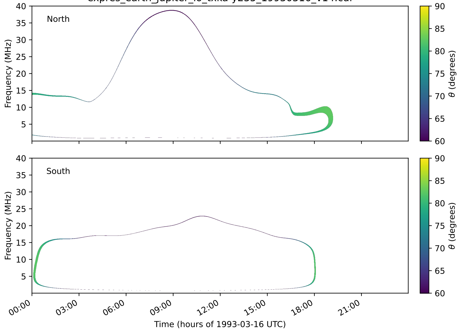
expres_earth_jupiter_io_txka-y235_19930316_v14.cdf
