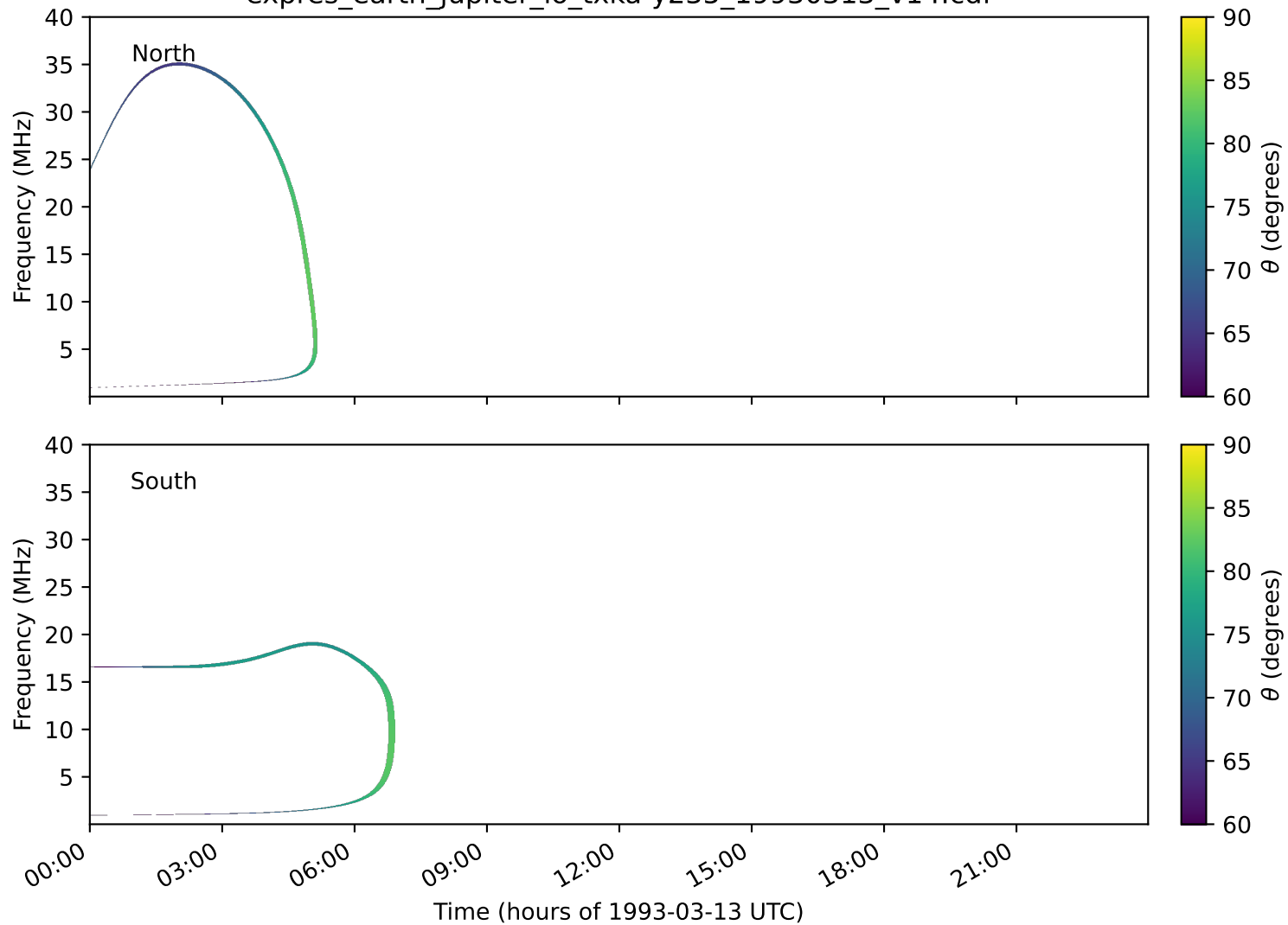
expres_earth_jupiter_io_txka-y235_19930313_v14.cdf
