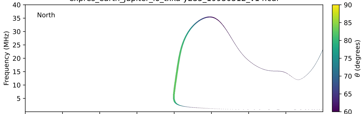
expres_earth_jupiter_io_txka-y235_19930312_v14.cdf
