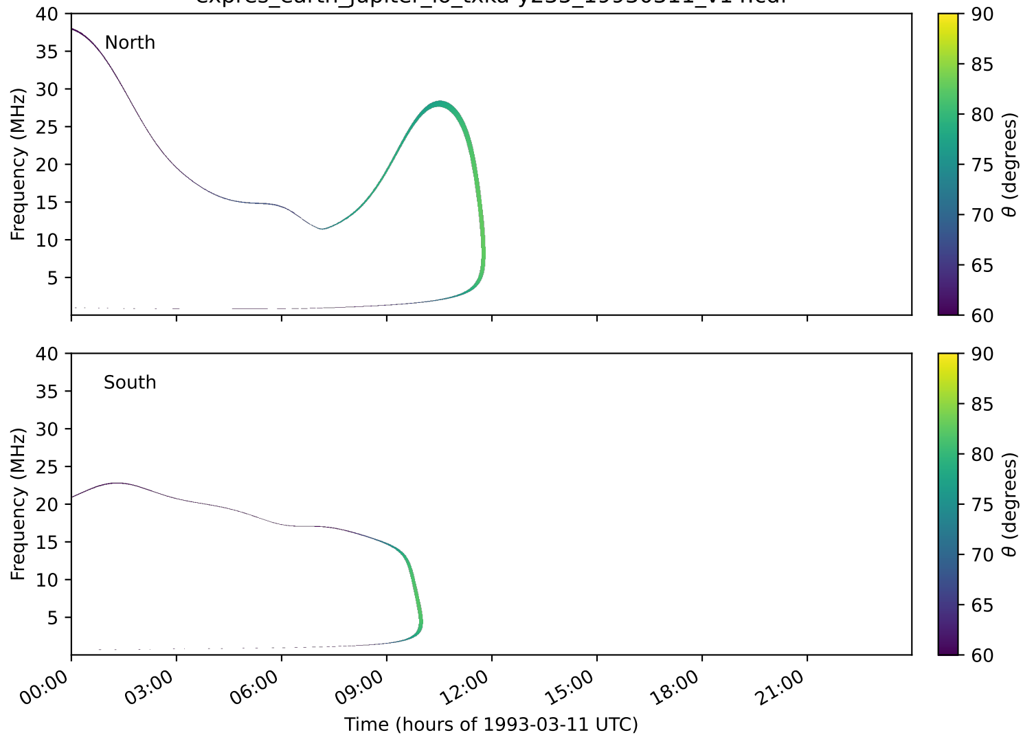
expres_earth_jupiter_io_txka-y235_19930311_v14.cdf
