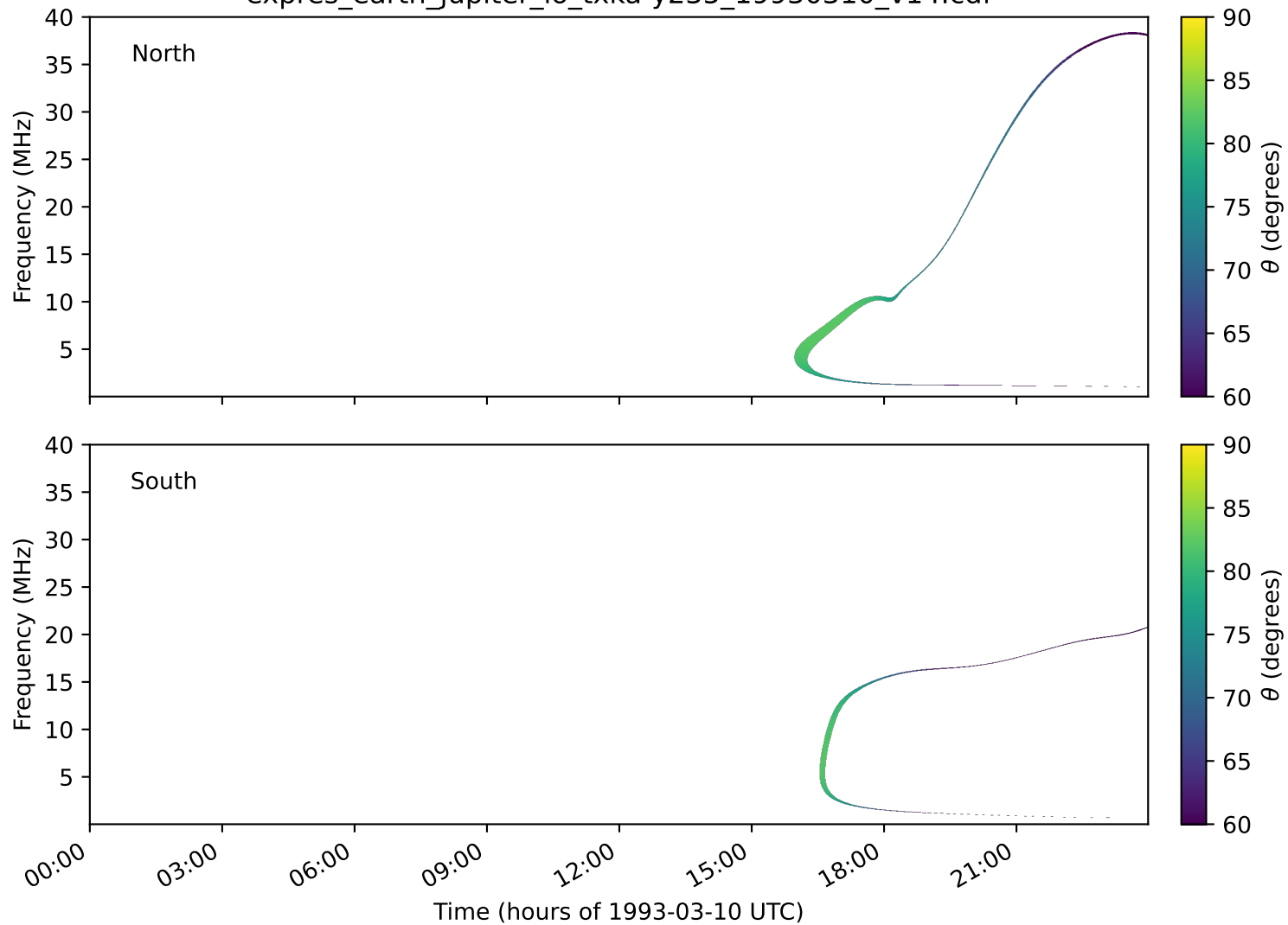
expres_earth_jupiter_io_txka-y235_19930310_v14.cdf
