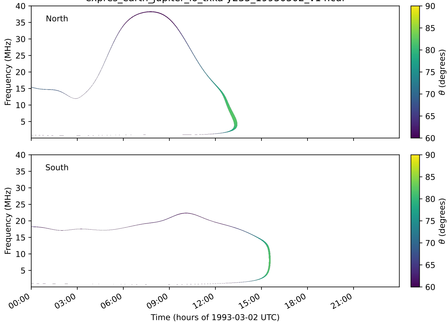
expres_earth_jupiter_io_txka-y235_19930302_v14.cdf
