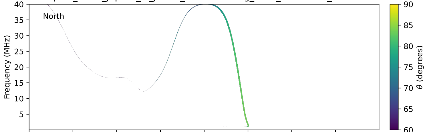
expres_earth_jupiter_io_jrm33_lossc-wid1deg_3kev_19930325_v11.cdf
