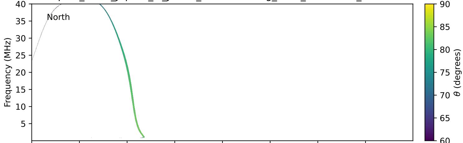
expres_earth_jupiter_io_jrm33_lossc-wid1deg_3kev_19930320_v11.cdf
