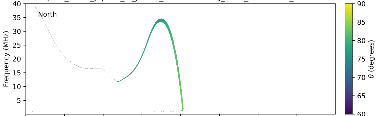
expres_earth_jupiter_io_jrm33_lossc-wid1deg_3kev_19930311_v11.cdf
