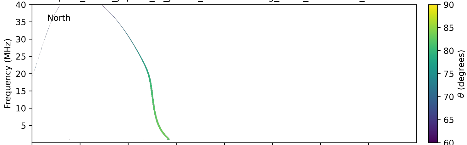
expres_earth_jupiter_io_jrm09_lossc-wid1deg_3kev_19930327_v11.cdf
