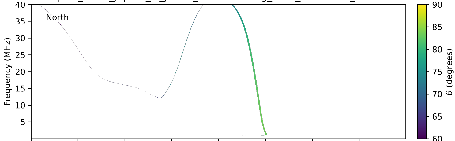
expres_earth_jupiter_io_jrm09_lossc-wid1deg_3kev_19930325_v11.cdf
