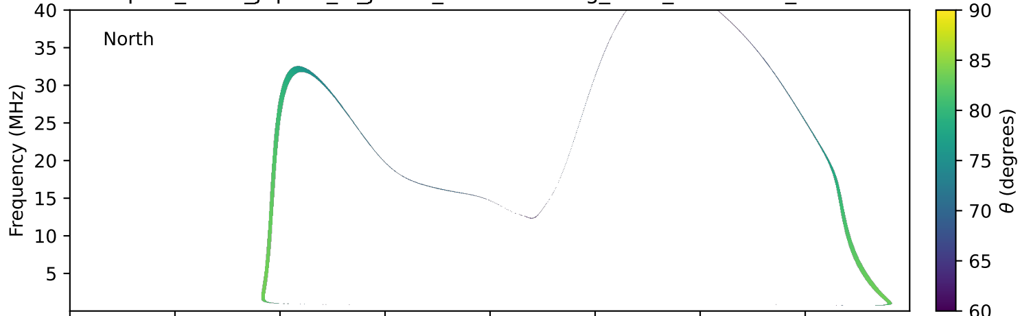
expres_earth_jupiter_io_jrm09_lossc-wid1deg_3kev_19930314_v11.cdf
