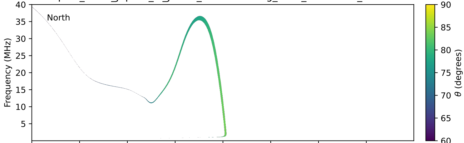
expres_earth_jupiter_io_jrm09_lossc-wid1deg_3kev_19930311_v11.cdf
