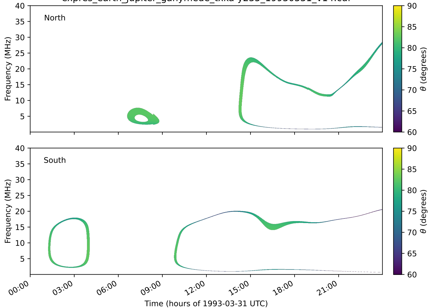
expres_earth_jupiter_ganymede_txka-y235_19930331_v14.cdf
