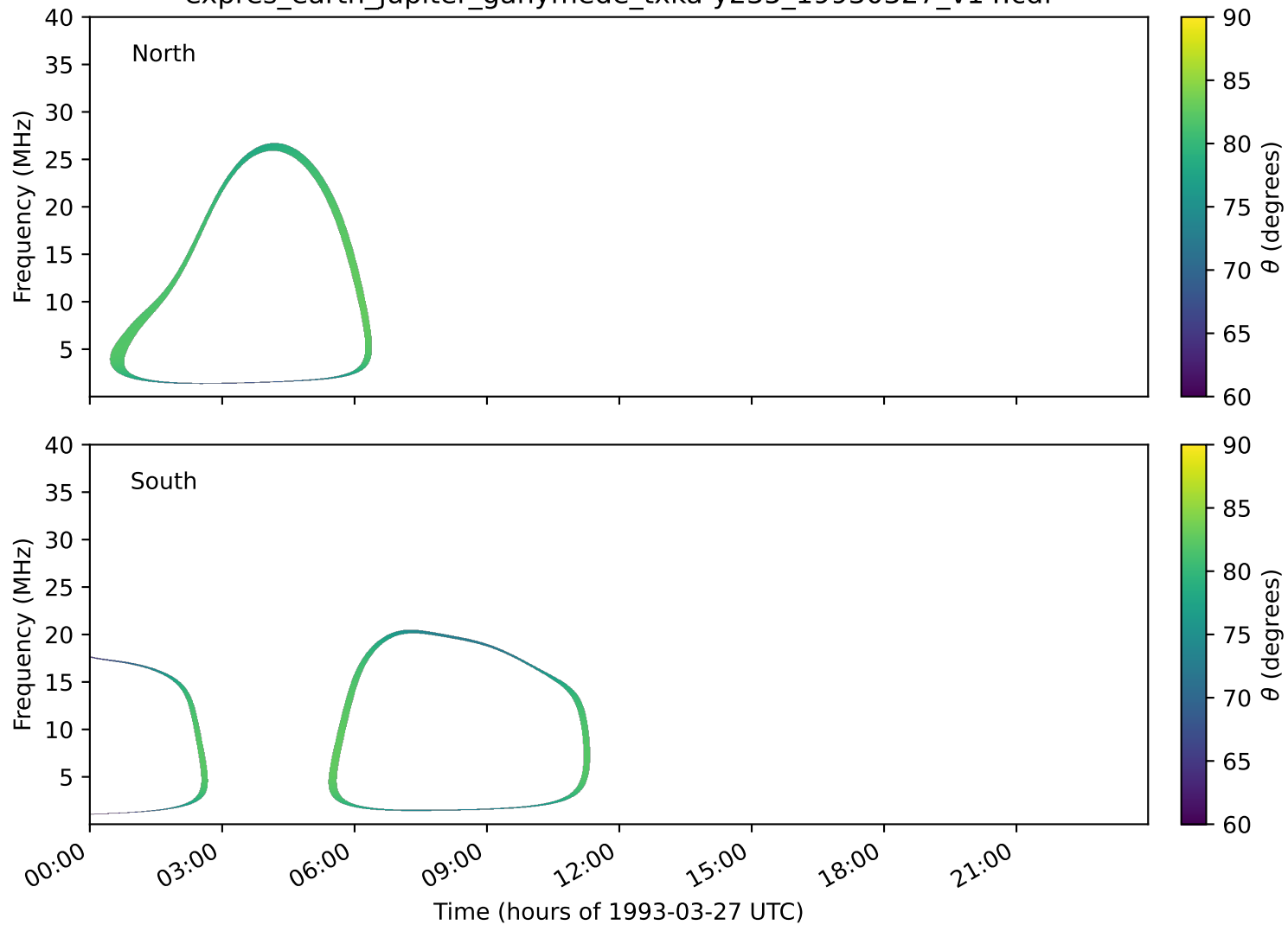
expres_earth_jupiter_ganymede_txka-y235_19930327_v14.cdf
