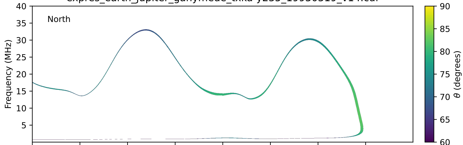
expres_earth_jupiter_ganymede_txka-y235_19930319_v14.cdf
