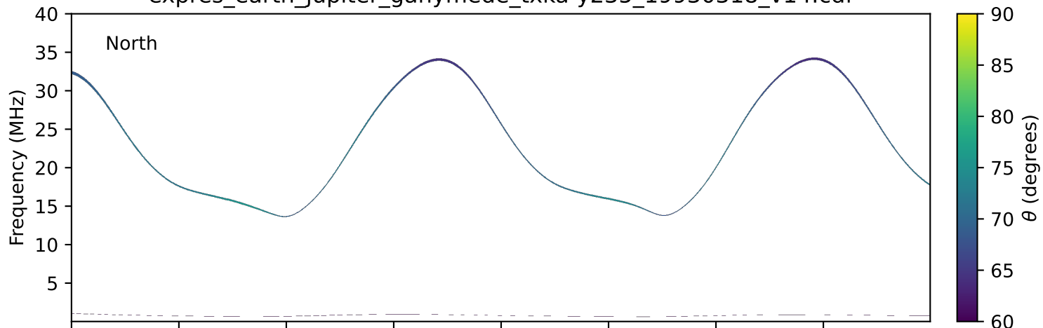
expres_earth_jupiter_ganymede_txka-y235_19930318_v14.cdf
