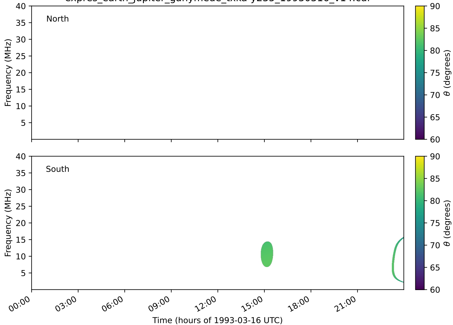
expres_earth_jupiter_ganymede_txka-y235_19930316_v14.cdf
