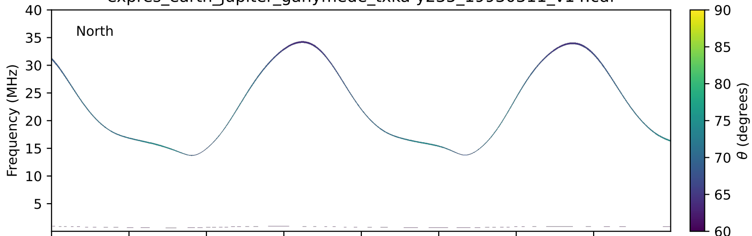
expres_earth_jupiter_ganymede_txka-y235_19930311_v14.cdf
