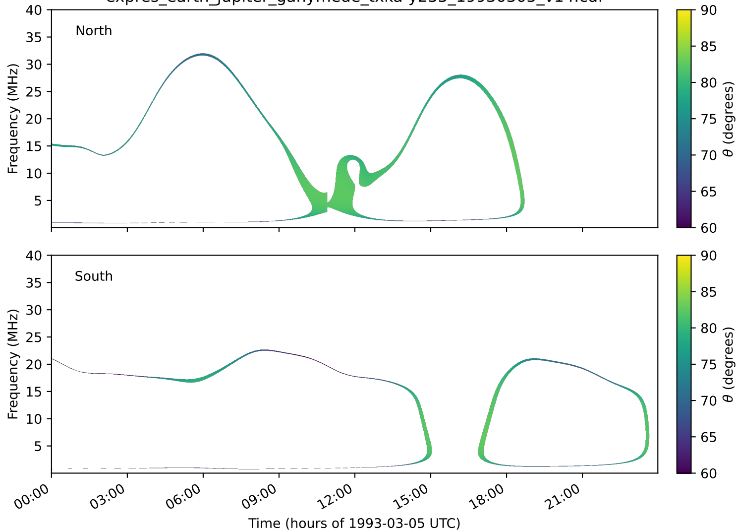
expres_earth_jupiter_ganymede_txka-y235_19930305_v14.cdf
