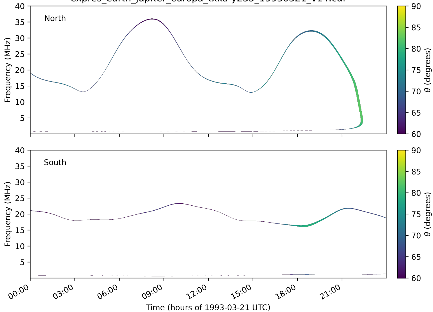
expres_earth_jupiter_europa_txka-y235_19930321_v14.cdf
