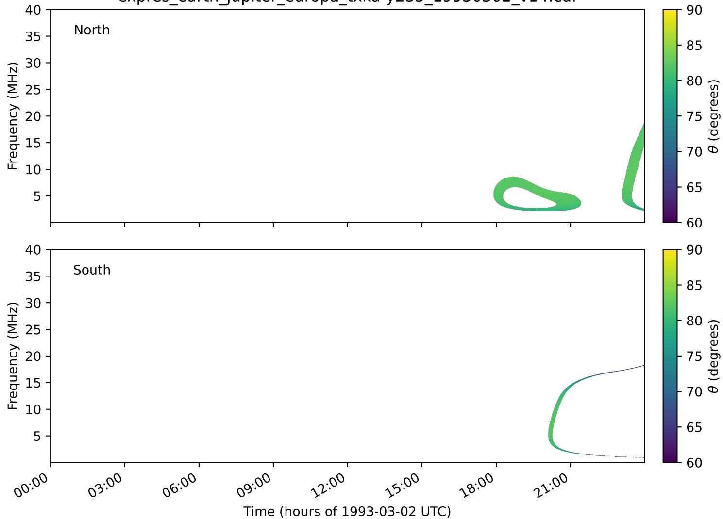
expres_earth_jupiter_europa_txka-y235_19930302_v14.cdf
