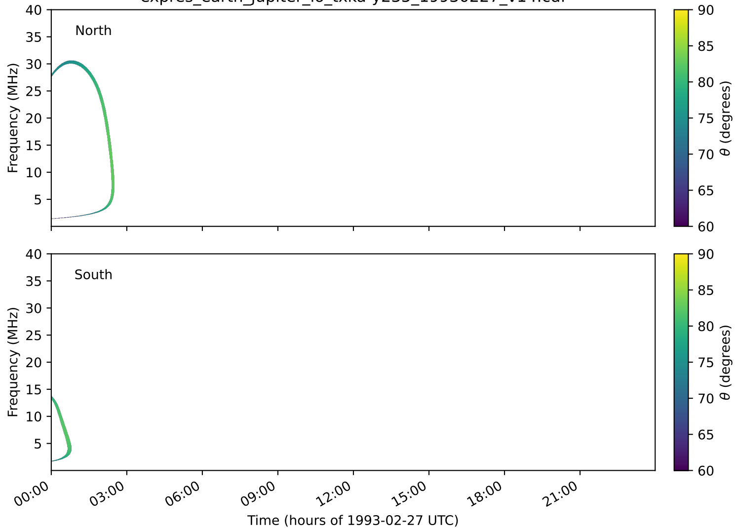
expres_earth_jupiter_io_txka-y235_19930227_v14.cdf
