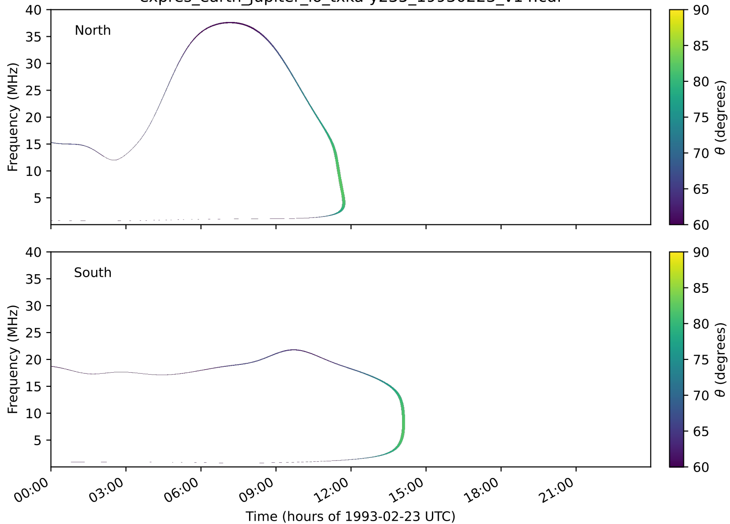
expres_earth_jupiter_io_txka-y235_19930223_v14.cdf
