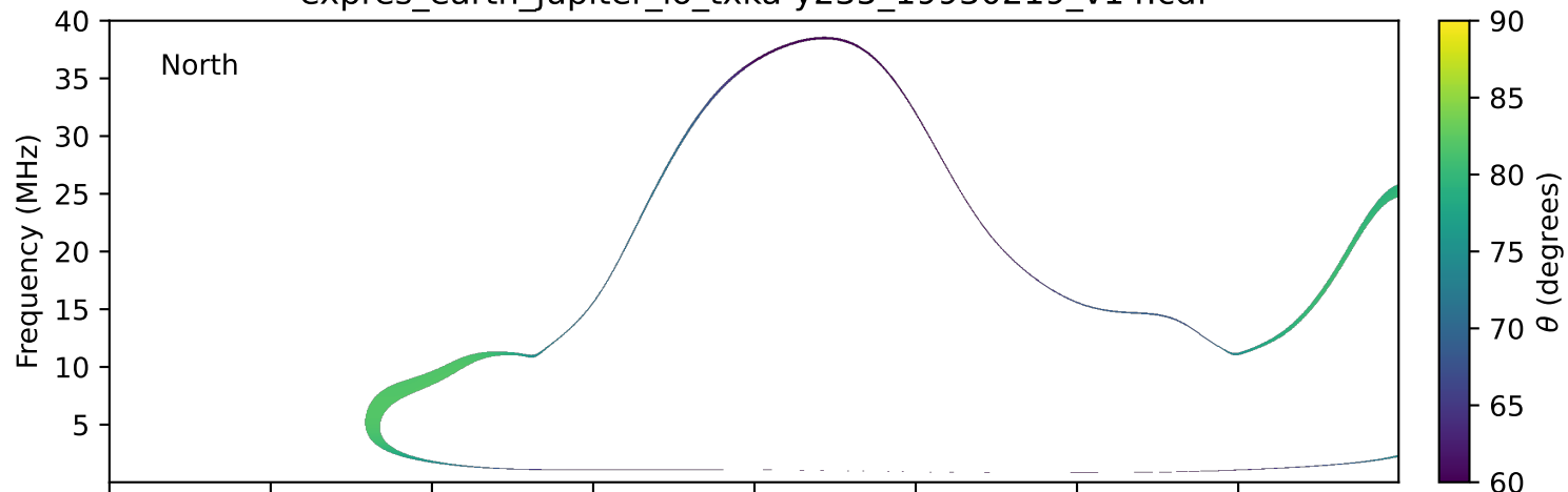
expres_earth_jupiter_io_txka-y235_19930219_v14.cdf
