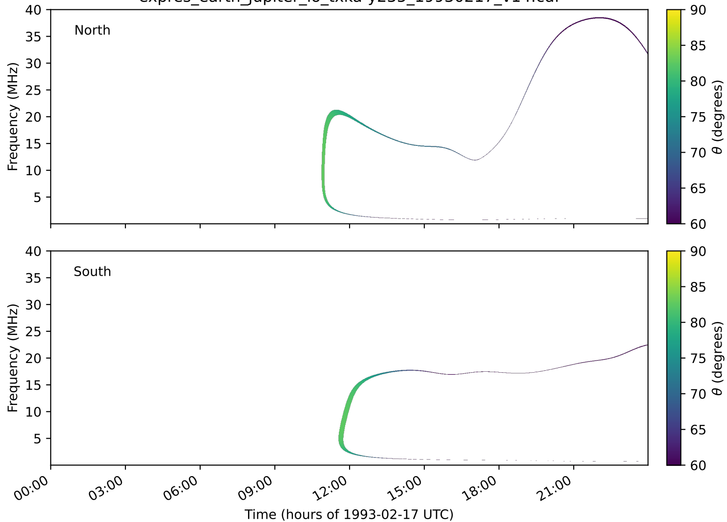
expres_earth_jupiter_io_txka-y235_19930217_v14.cdf
