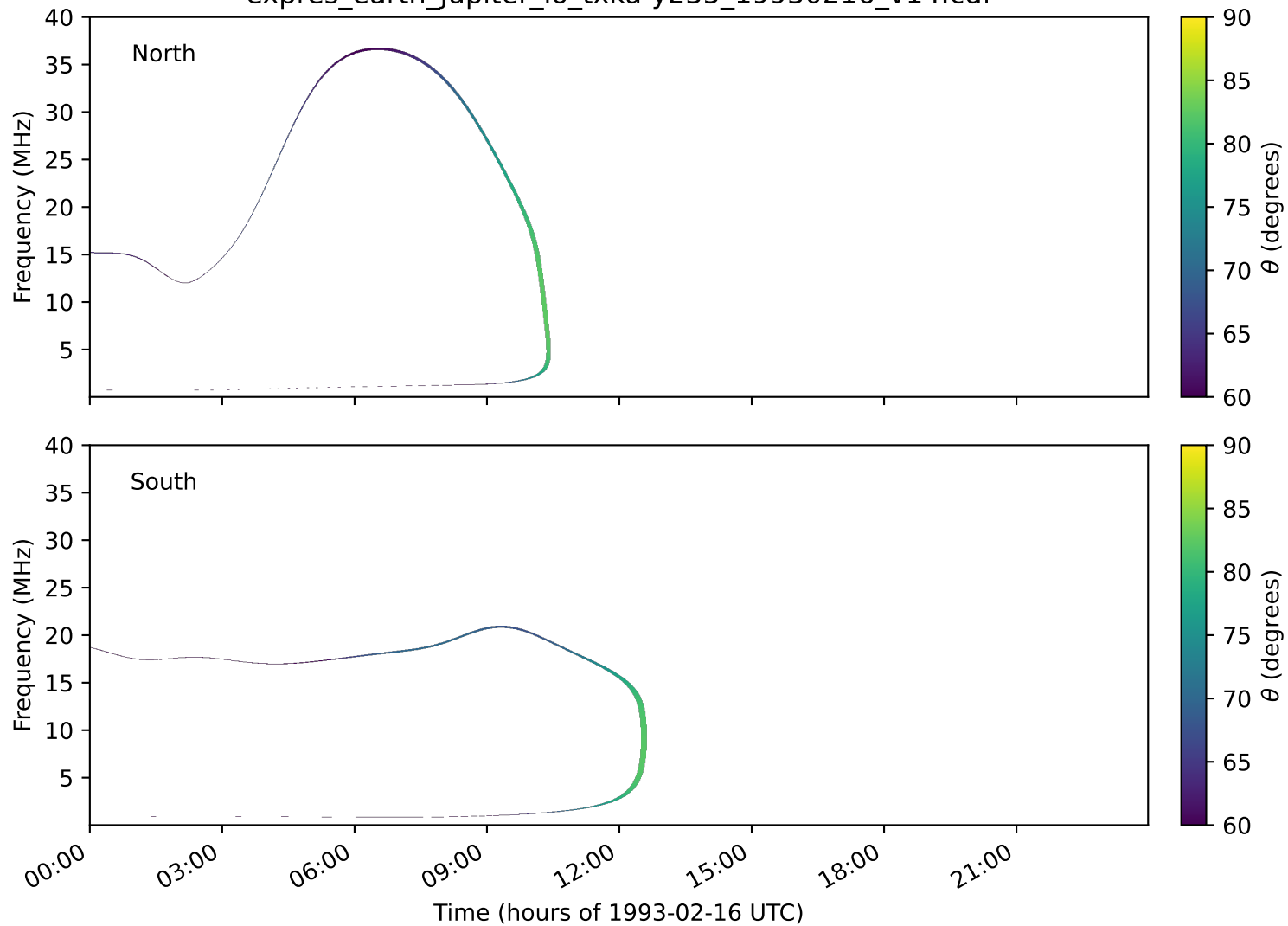
expres_earth_jupiter_io_txka-y235_19930216_v14.cdf
