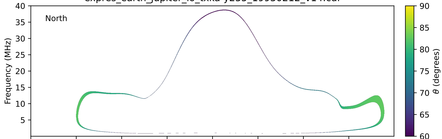
expres_earth_jupiter_io_txka-y235_19930212_v14.cdf
