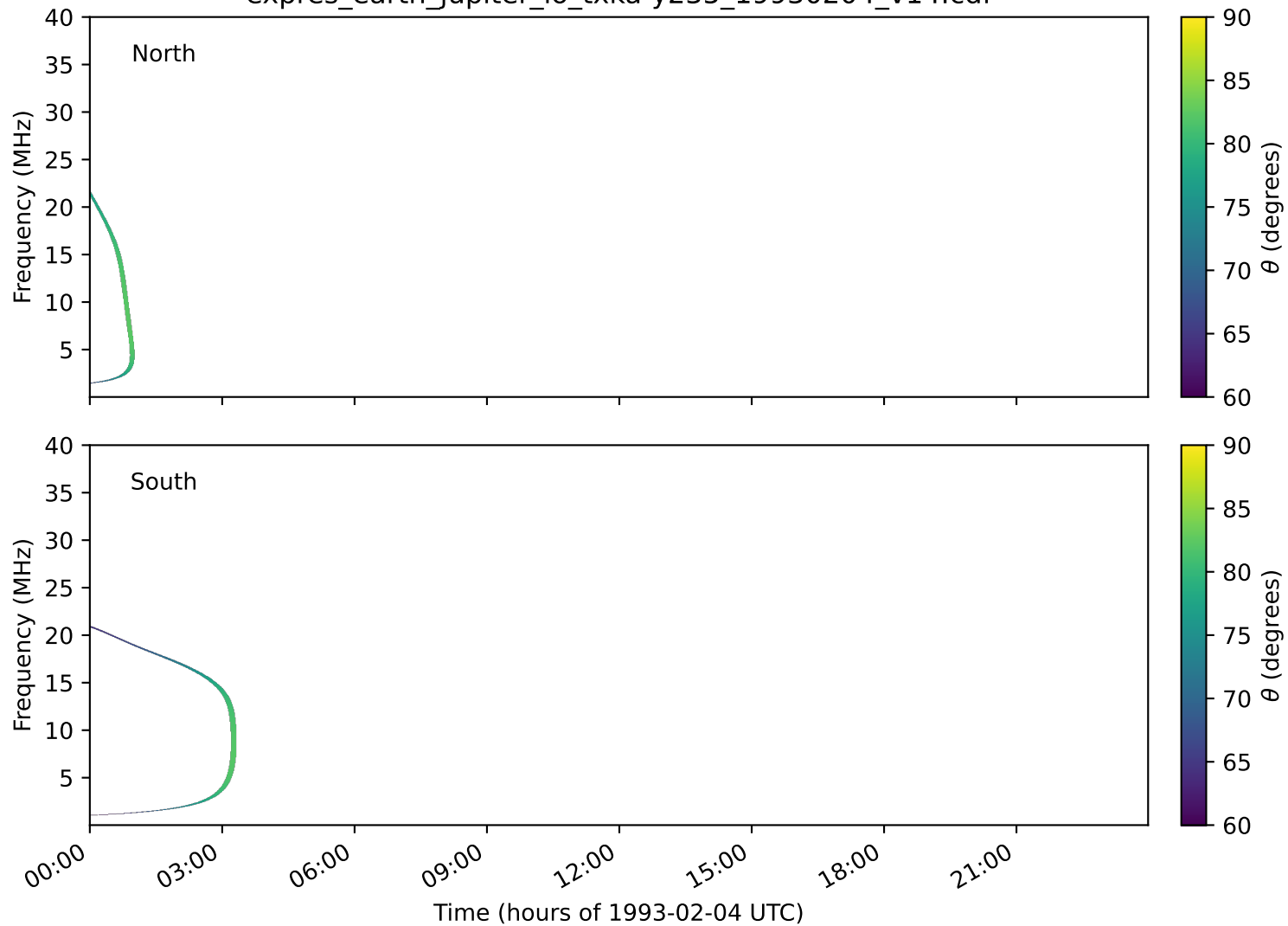
expres_earth_jupiter_io_txka-y235_19930204_v14.cdf
