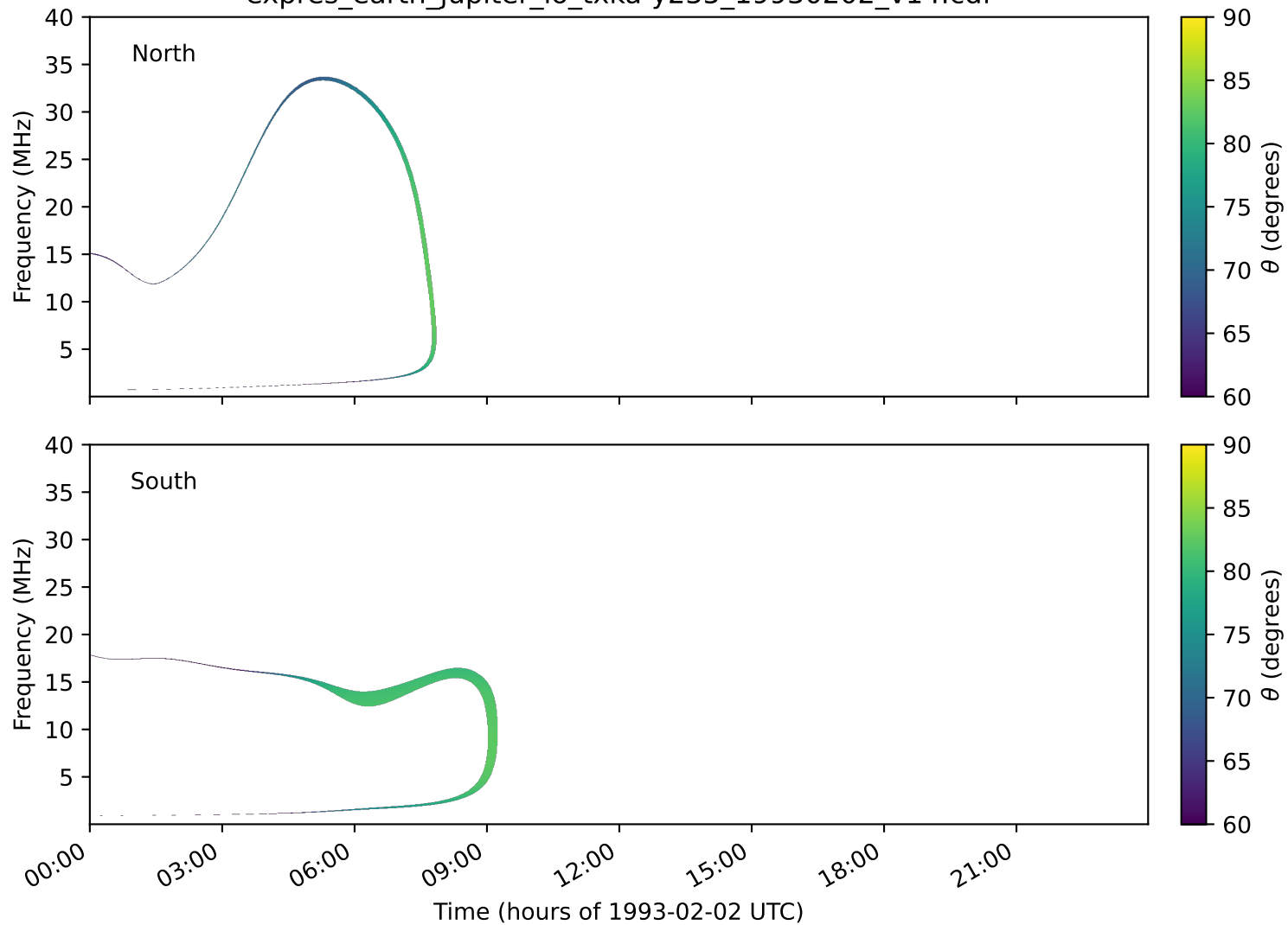
expres_earth_jupiter_io_txka-y235_19930202_v14.cdf
