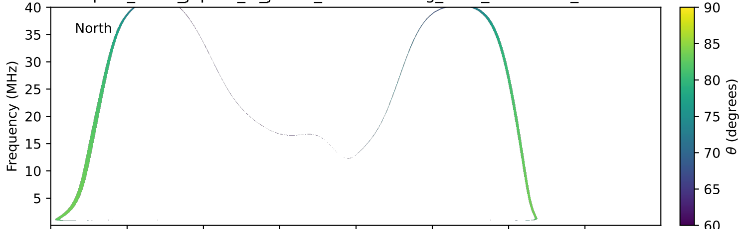
expres_earth_jupiter_io_jrm33_lossc-wid1deg_3kev_19930221_v11.cdf
