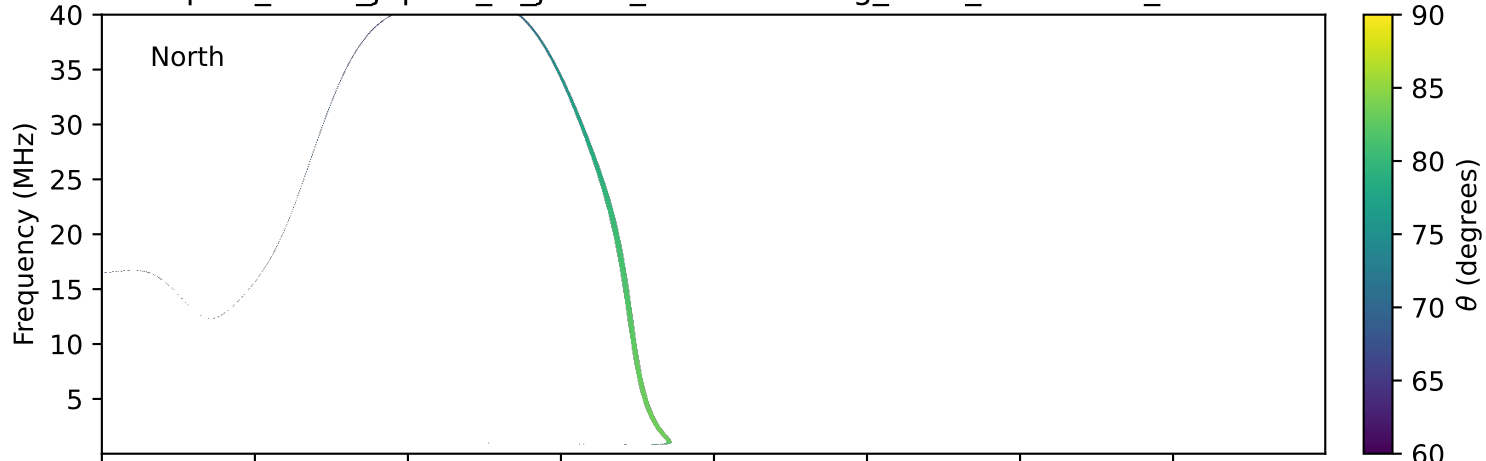
expres_earth_jupiter_io_jrm33_lossc-wid1deg_3kev_19930216_v11.cdf
