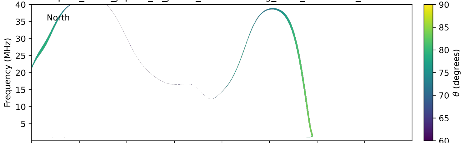
expres_earth_jupiter_io_jrm33_lossc-wid1deg_3kev_19930214_v11.cdf
