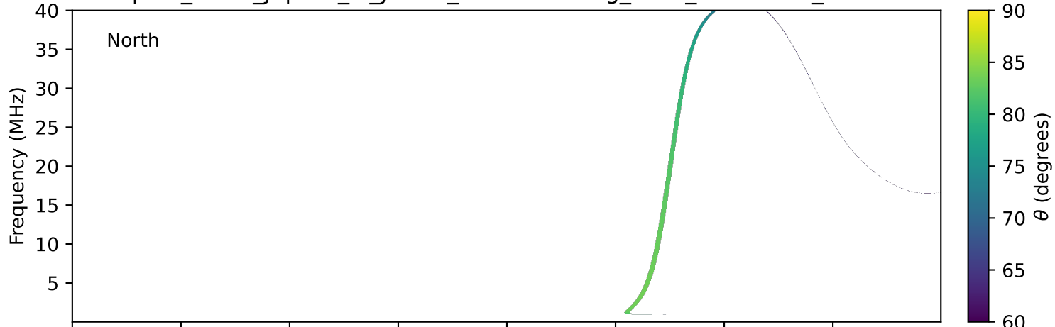
expres_earth_jupiter_io_jrm33_lossc-wid1deg_3kev_19930208_v11.cdf
