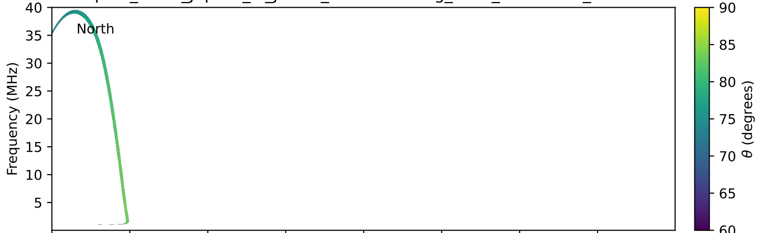
expres_earth_jupiter_io_jrm09_lossc-wid1deg_3kev_19930227_v11.cdf
