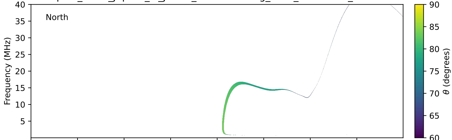
expres_earth_jupiter_io_jrm09_lossc-wid1deg_3kev_19930224_v11.cdf
