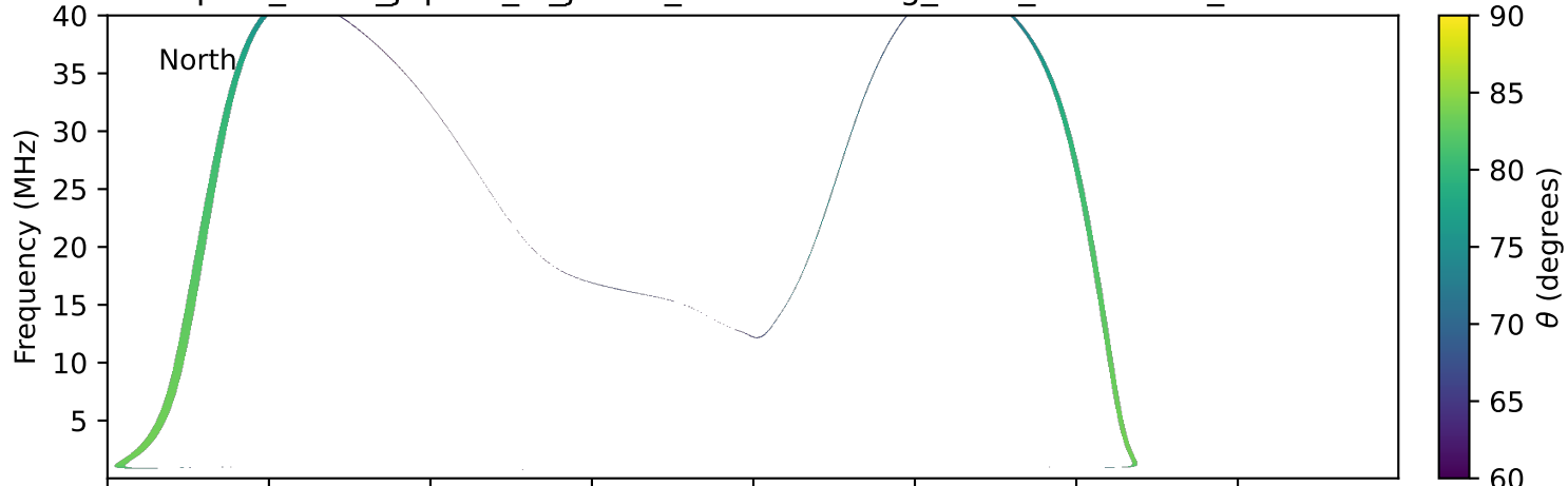
expres_earth_jupiter_io_jrm09_lossc-wid1deg_3kev_19930221_v11.cdf
