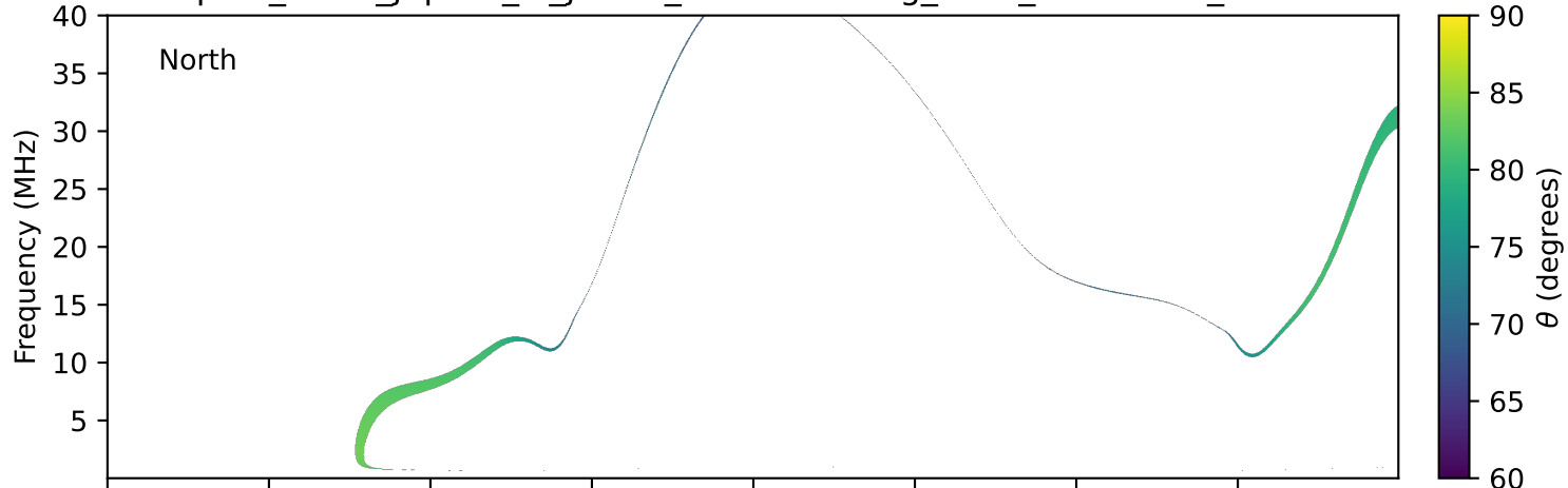
expres_earth_jupiter_io_jrm09_lossc-wid1deg_3kev_19930219_v11.cdf
