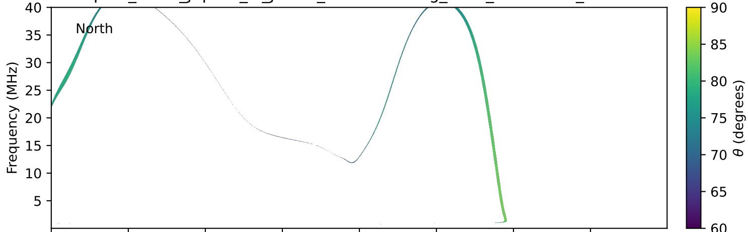
expres_earth_jupiter_io_jrm09_lossc-wid1deg_3kev_19930214_v11.cdf
