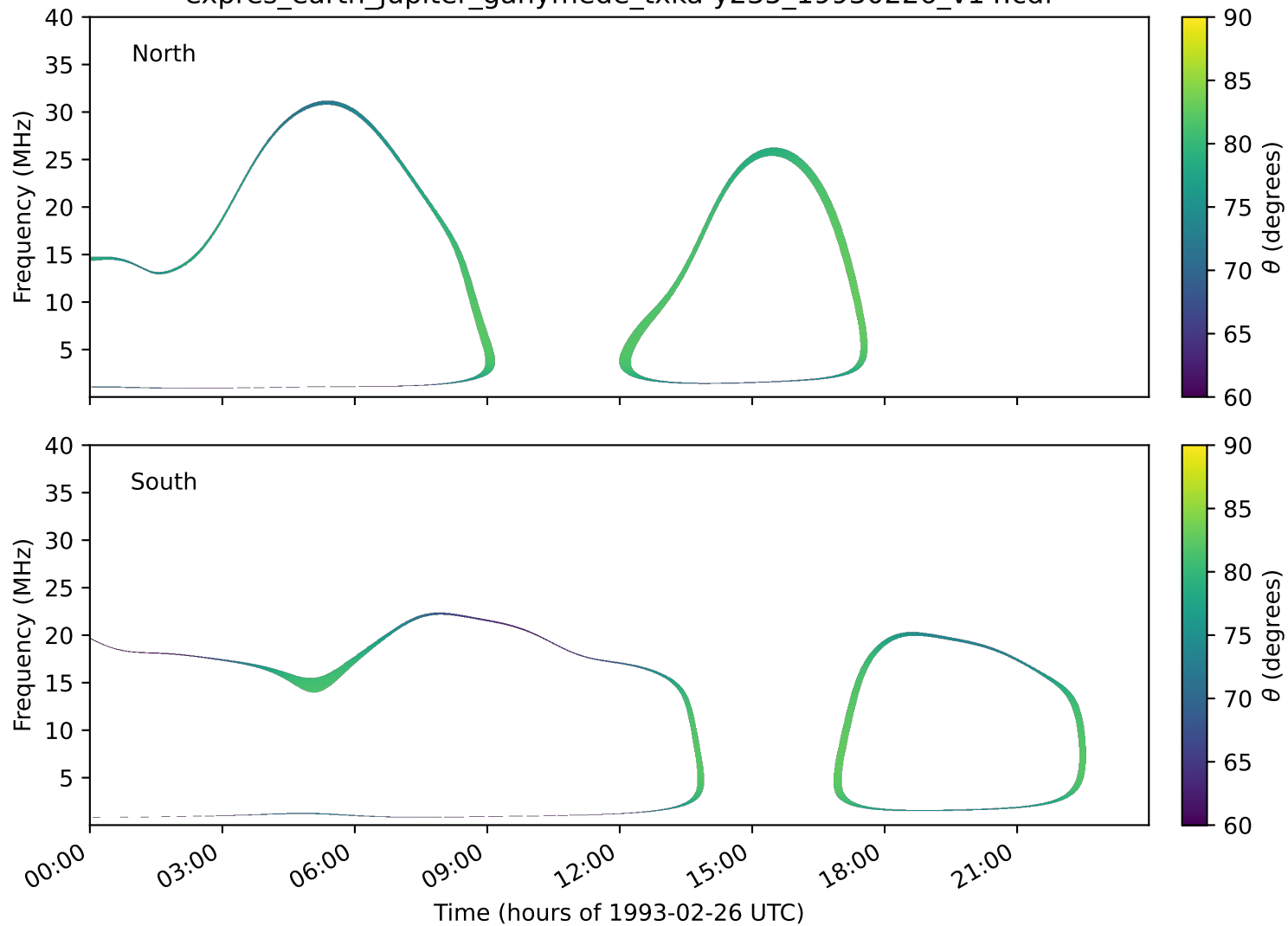
expres_earth_jupiter_ganymede_txka-y235_19930226_v14.cdf
