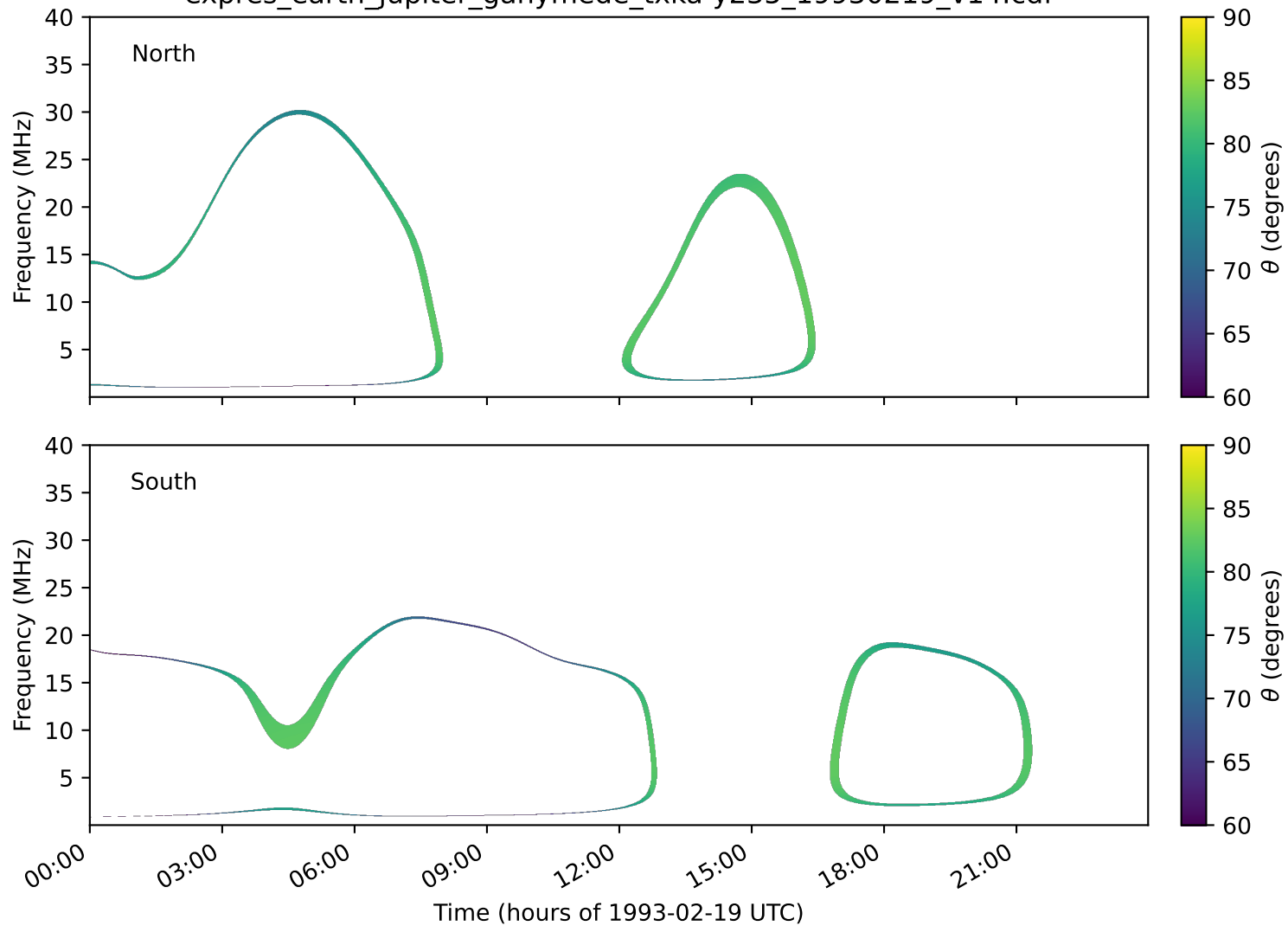
expres_earth_jupiter_ganymede_txka-y235_19930219_v14.cdf
