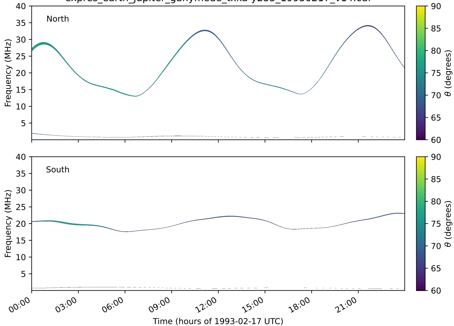
expres_earth_jupiter_ganymede_txka-y235_19930217_v14.cdf
