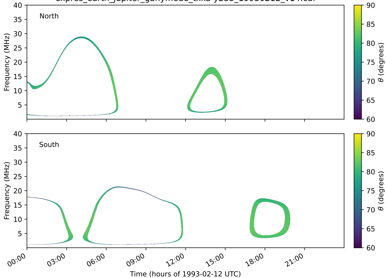
expres_earth_jupiter_ganymede_txka-y235_19930212_v14.cdf
