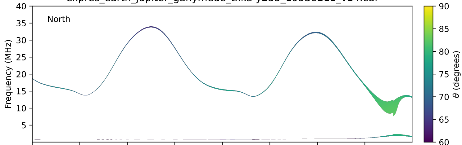
expres_earth_jupiter_ganymede_txka-y235_19930211_v14.cdf
