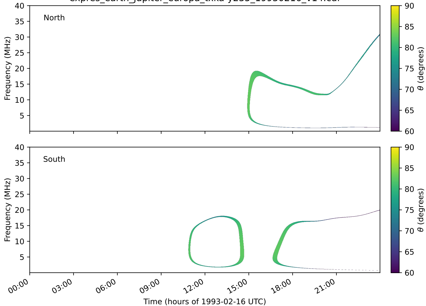
expres_earth_jupiter_europa_txka-y235_19930216_v14.cdf
