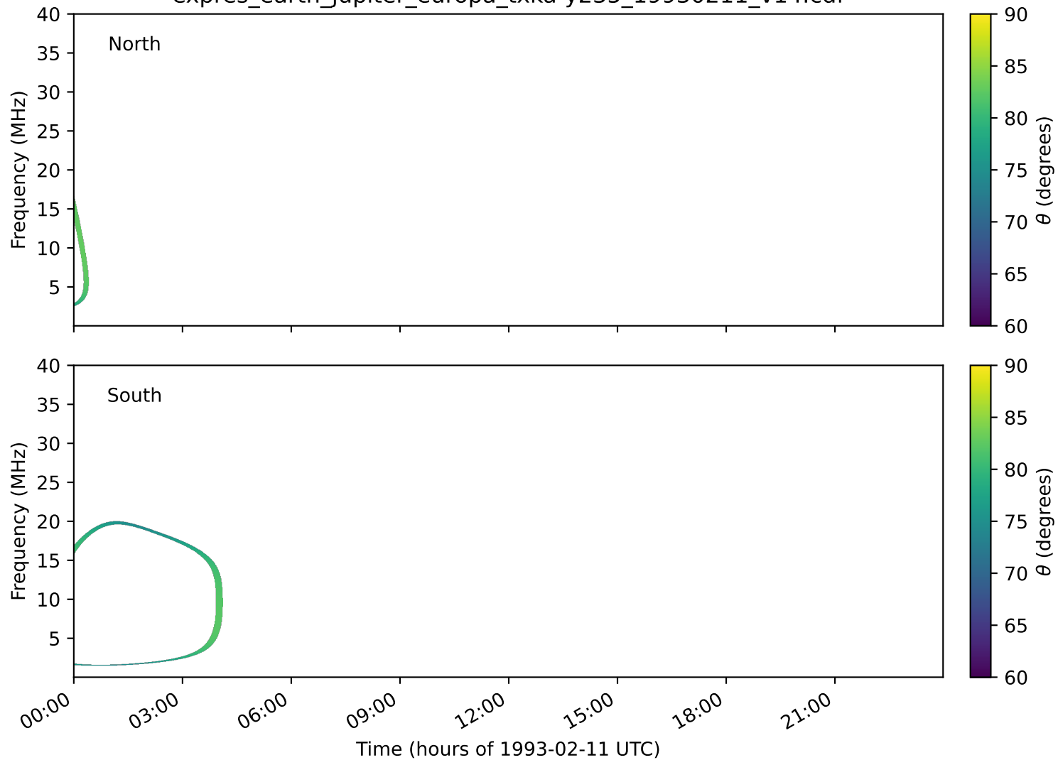
expres_earth_jupiter_europa_txka-y235_19930211_v14.cdf
