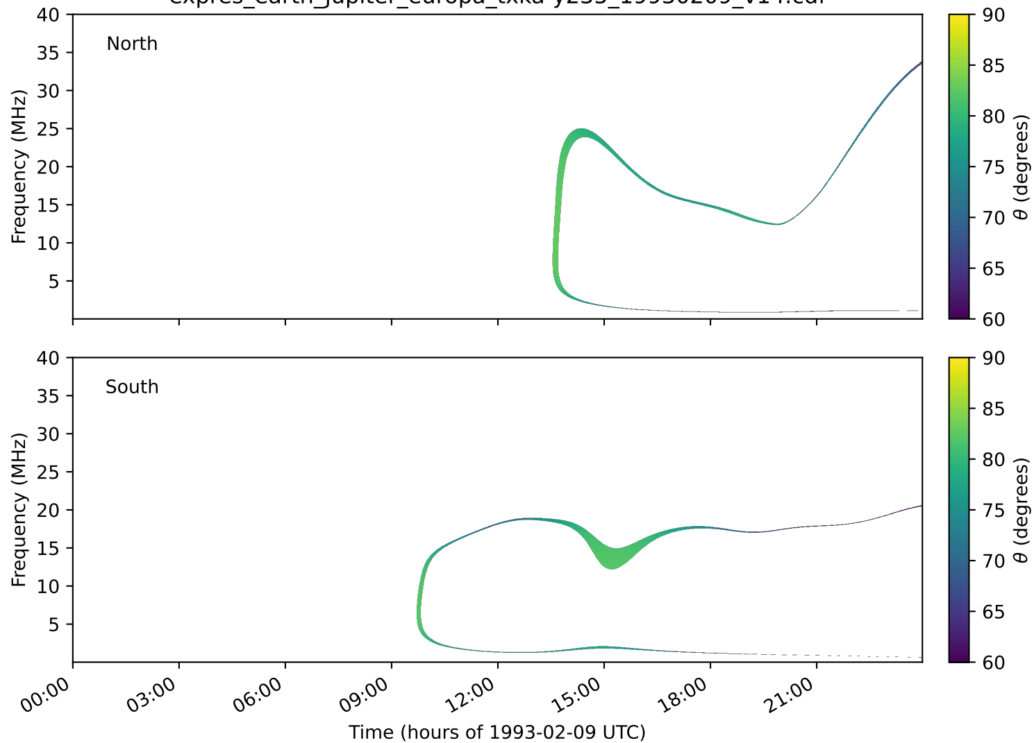
expres_earth_jupiter_europa_txka-y235_19930209_v14.cdf
