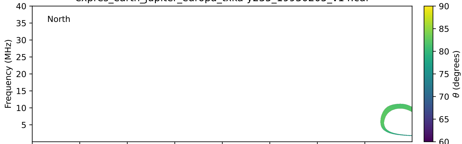
expres_earth_jupiter_europa_txka-y235_19930205_v14.cdf
