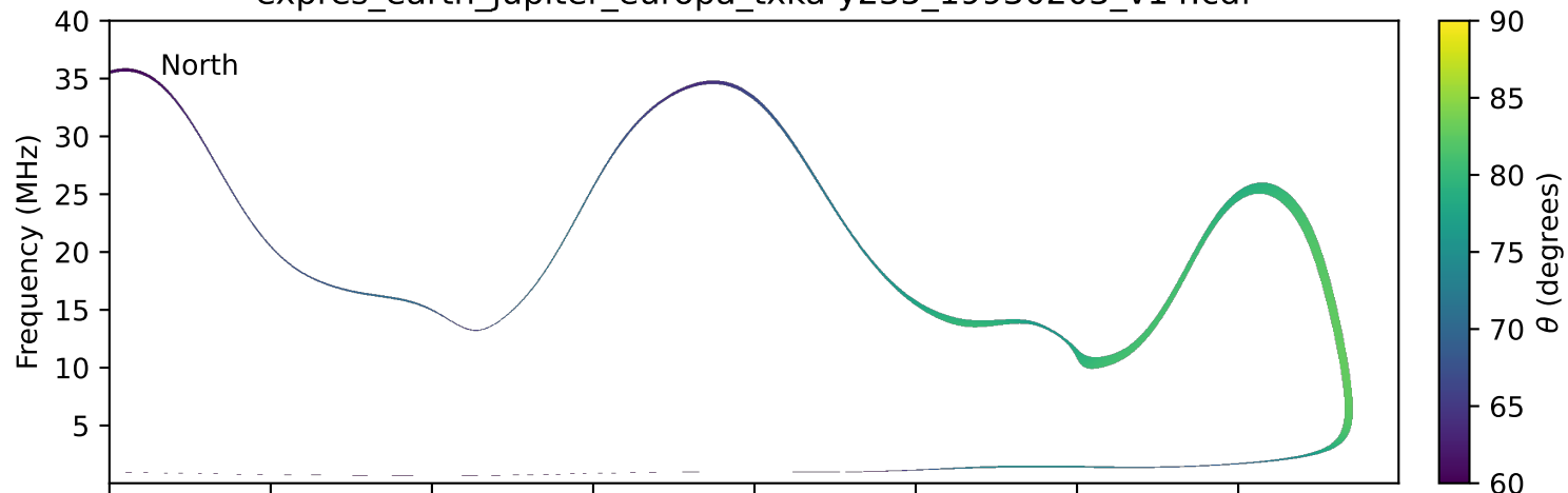
expres_earth_jupiter_europa_txka-y235_19930203_v14.cdf
