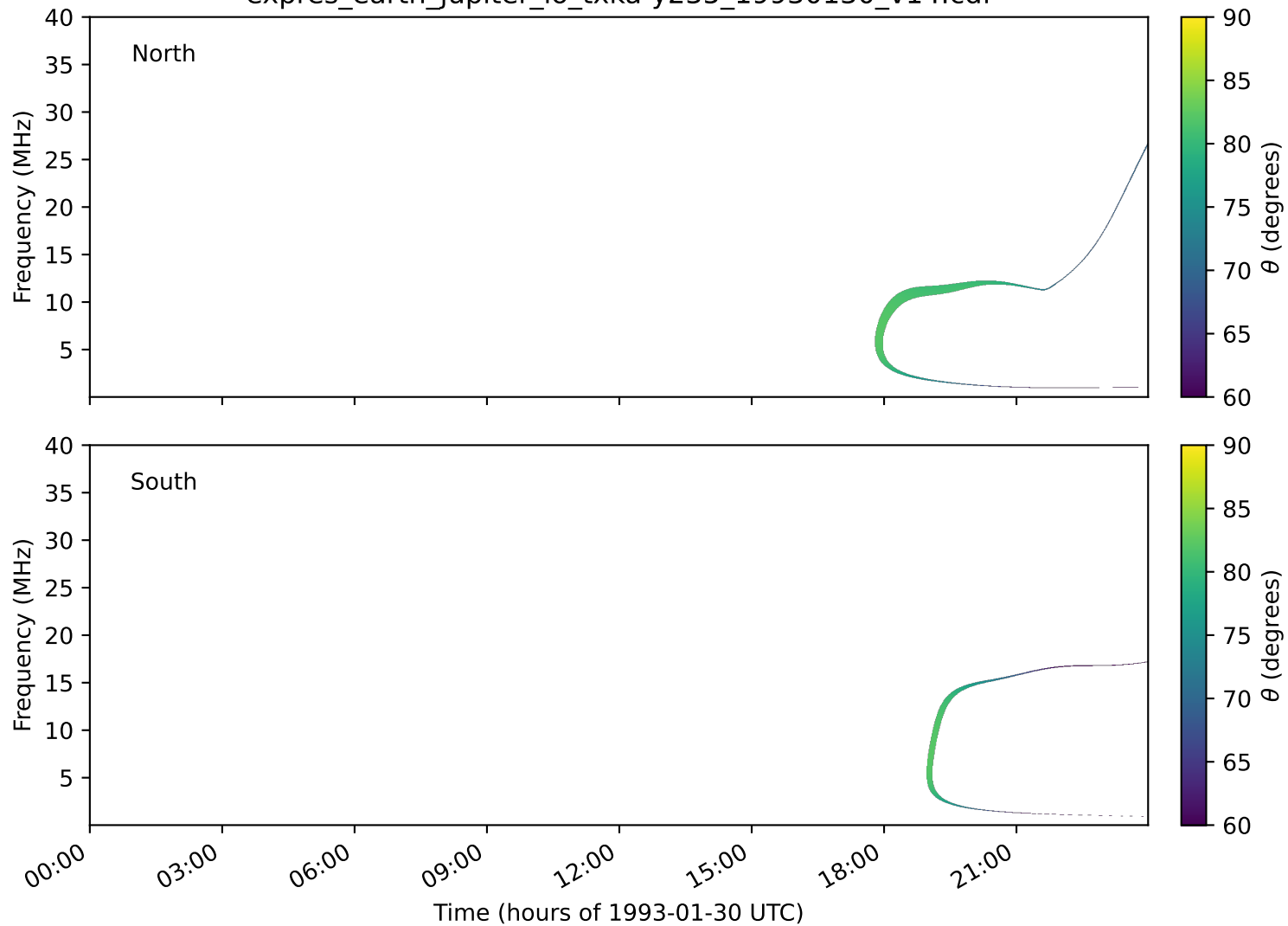
expres_earth_jupiter_io_txka-y235_19930130_v14.cdf
